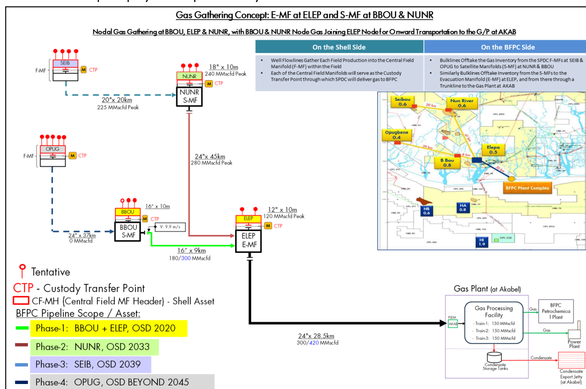
Figure 4.1: Feedstock & Products Evacuation Schematics
